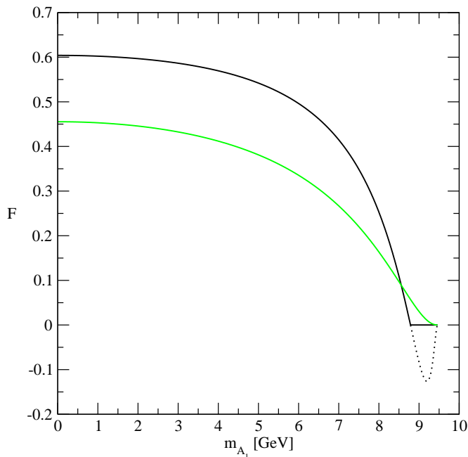
Figure 1: F(m_{A_1}) including the bound state and QCD corrections, and a naive extrapolation of the relativistic corrections computed for m_{A_1} \ll m_\gamma at larger values of m_{A_1} . Black curve: assuming m_b = 4.9 GeV (as used later), green curve: assuming m_b = 5.3 GeV.
