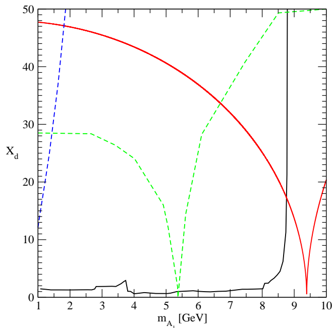
Figure 3: Upper bounds on X_d versus the A_1 mass for all parameters scanned over (see text). Indicated are constraints from B_s \rightarrow \mu^+\mu^- and \Delta M_q , q = d, s as a green dashed line, constraints from (g-2)_\mu as a blue dashed line, the latest bounds from CLEO on \mathcal{B}(\Upsilon \rightarrow \gamma\tau\tau) as a black line and constraints due to the measured \eta_b(1S) mass by Babar as a red line.
